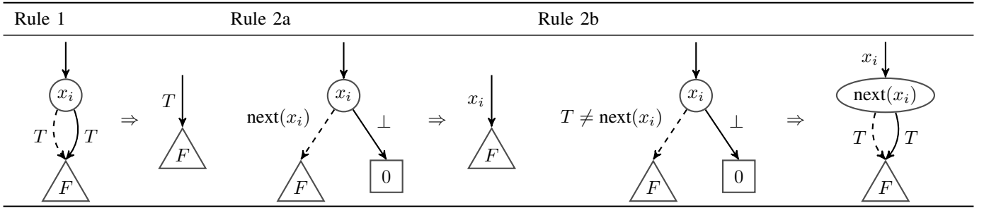
Fig. 5: The reduction rules of a TBDD for bottom-up reduction. Here T stands for any tag and F for any reduced TBDD; next(x) is the next variable in the variable domain, or \perp if x is the last variable.
